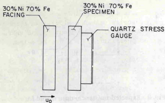
Fig. 10 Experimental arrangement for compressibility measurement on fcc 30%Ni-70%Fe
